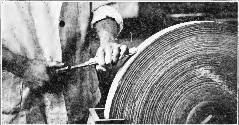
FIG. 123. GRINDING A TURNER'S GOUGE.
